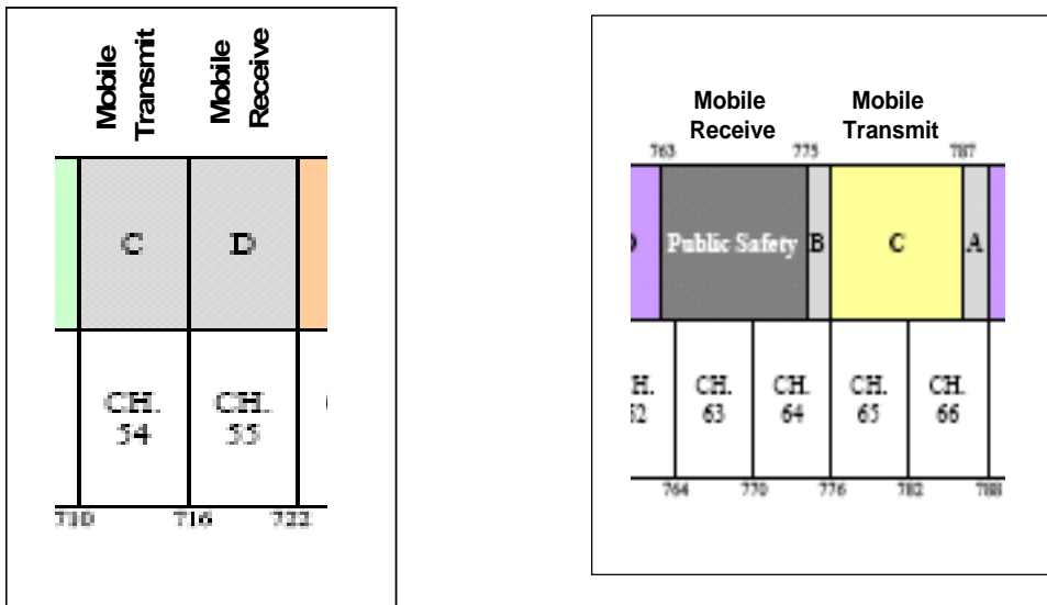
Figure 2: 700 MHz Adjacent Mobile-to-Mobile Operations
